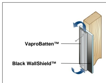
VaproBatten application drawing
