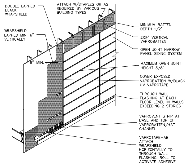
RAIN SCREEN OPEN JOINT -NARROW PANEL A.B.
